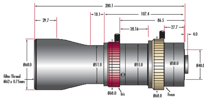
1X & 0.73X Telecentric Lenses
