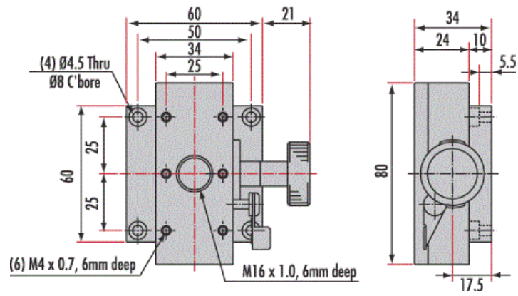
#55-026 - 60mm Travel, X-Axis Rack & Pinion Stage
