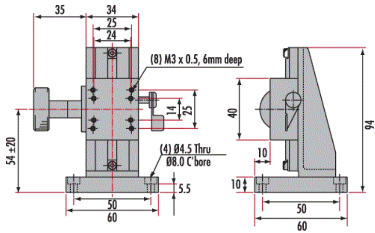
#55-024 - 40mm Z Travel, Z-Axis Rack & Pinion Stage
