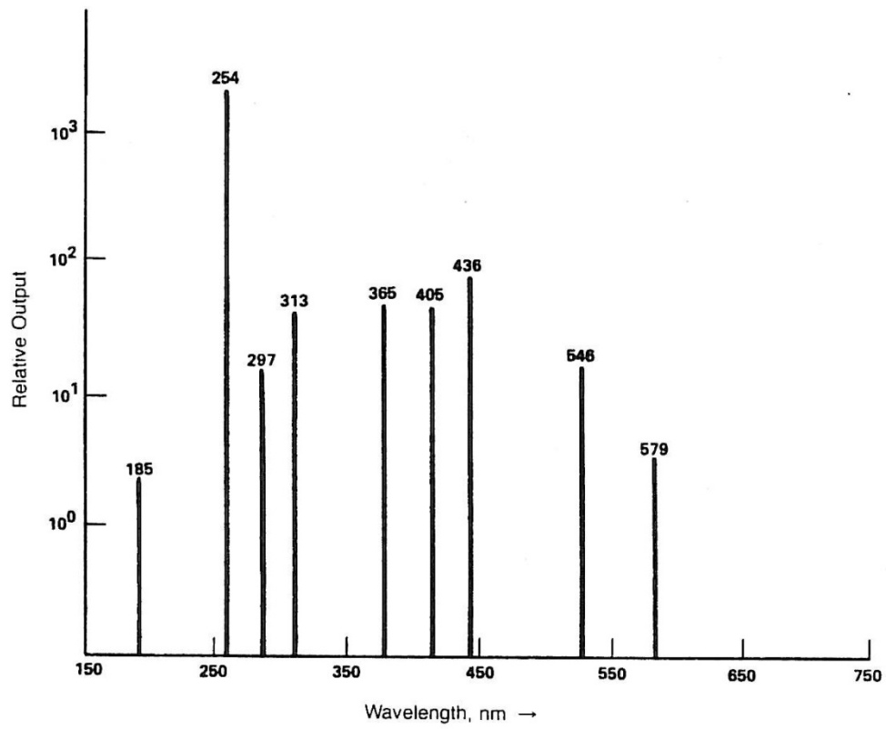
Figure 12: Typical Output From Low Pressure Mercury Lamp
