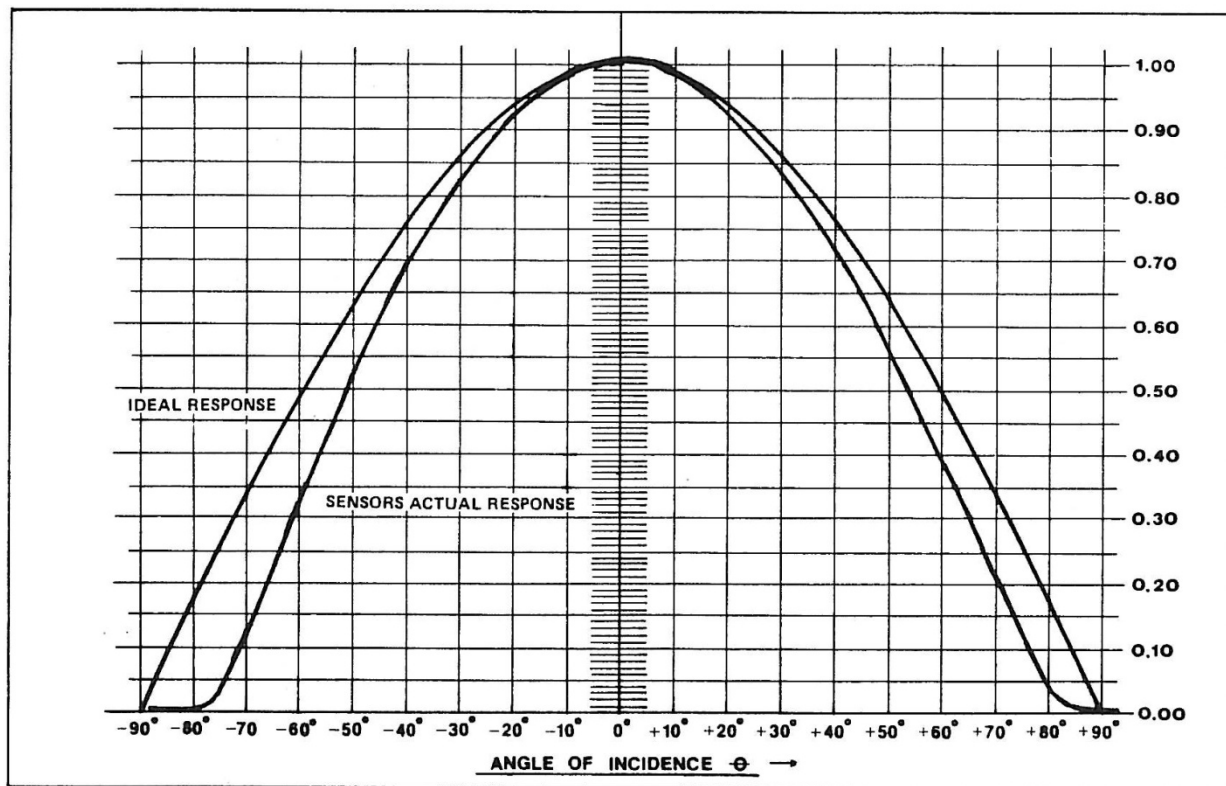
Figure 9: Typical Sensor Response Versus Incidence Angle
