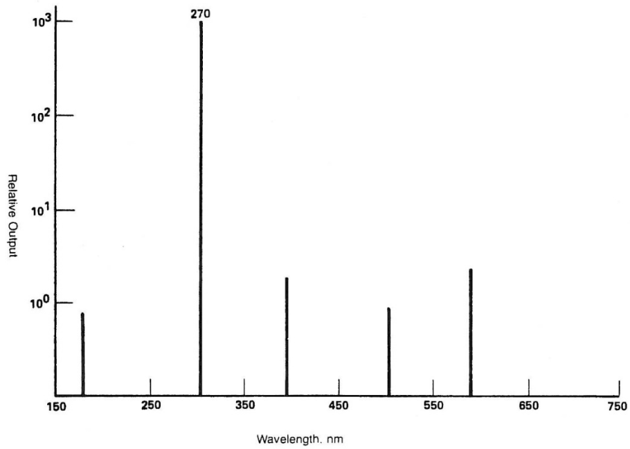
Figure 13: Hypothetical Light Source Having an Output at 270nm Wavelength
