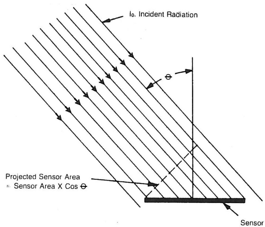
Figure 17: Projected Area of Sensor
