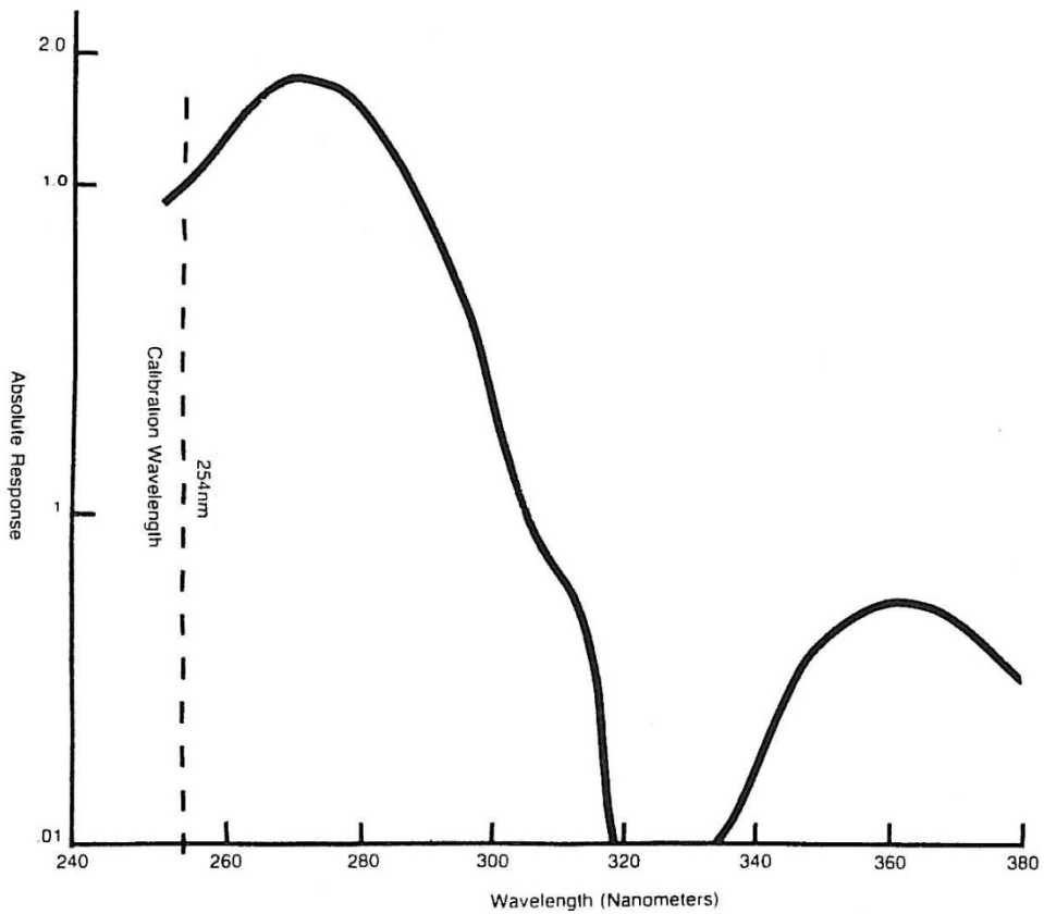
Figure 6: Typical UVX-25 Sensor Spectral Response
