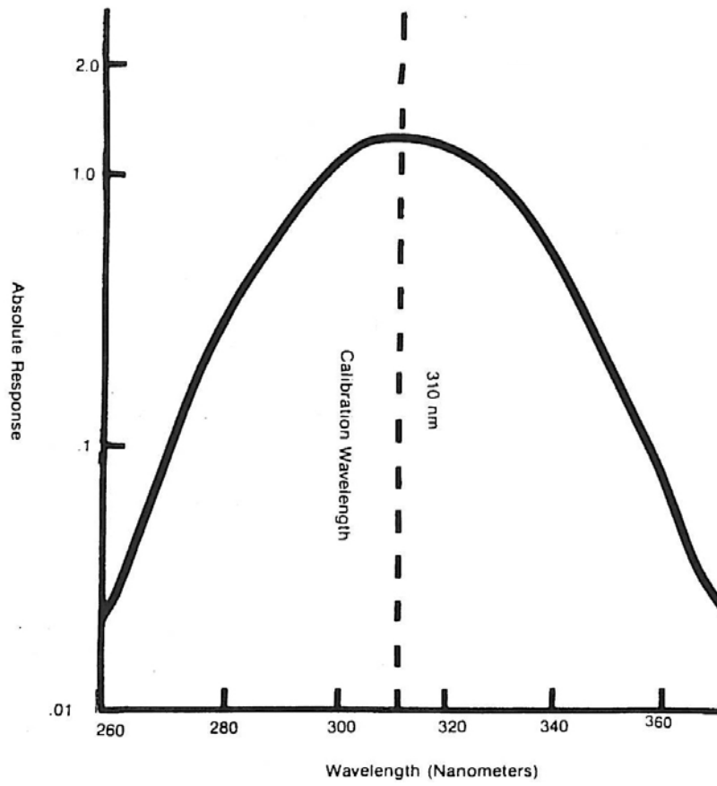
Figure 7: Typical UVX-31 Sensor Spectral Response
