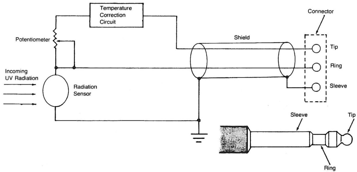
Figure 10: Schematic of UVX Series Sensor
