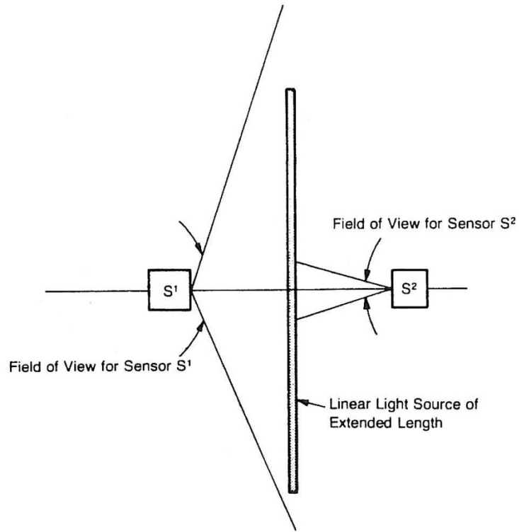
Figure 16: Example, Illustrating Why Sensor Field of View is Important When Measuring Irradiance
