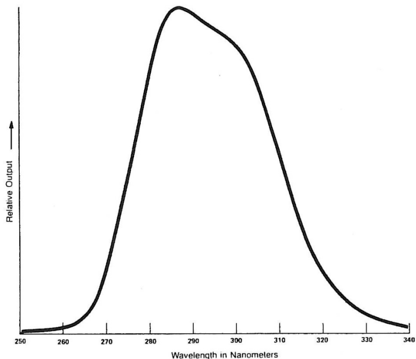
Figure 15: Continuous Emitter, 285nm Phosphor Coated UV Lamp
