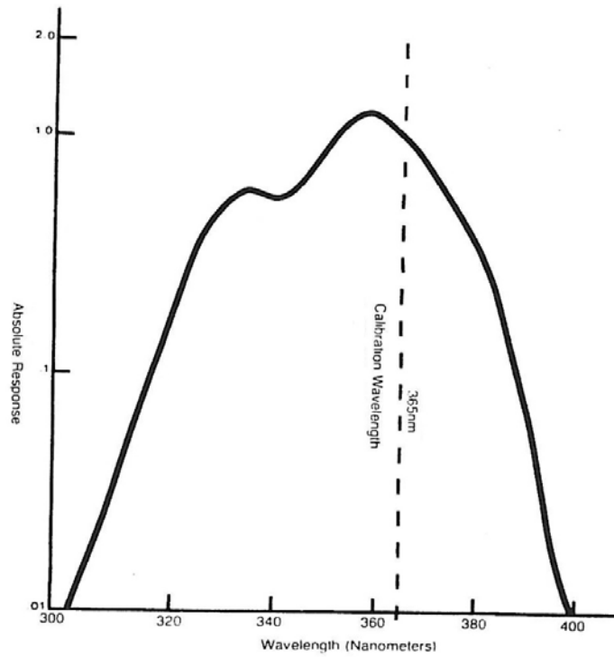
Figure 8: Typical UVX-36 Sensor Spectral Response
