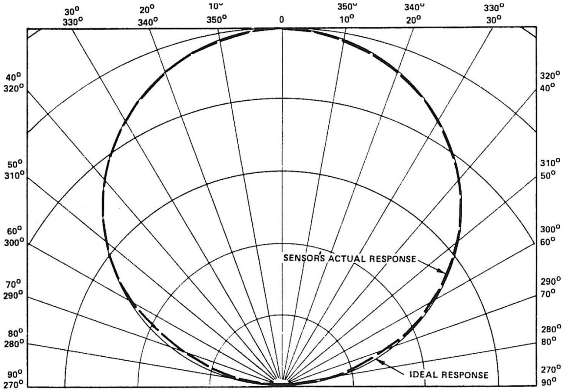
Figure 18: Cosine Response of Typical UVX Sensor (Polar Plot)
