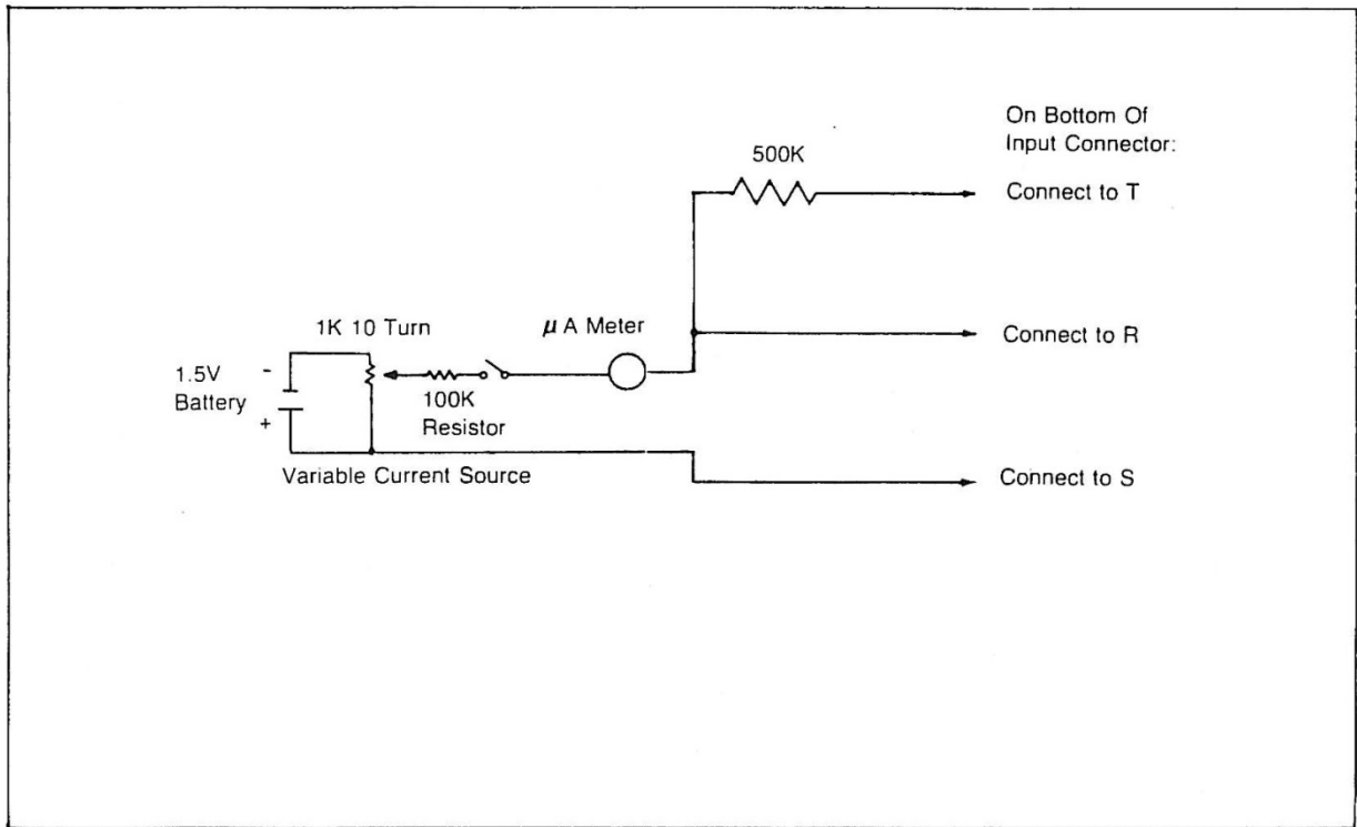
Figure 3: Calibration Current Source
