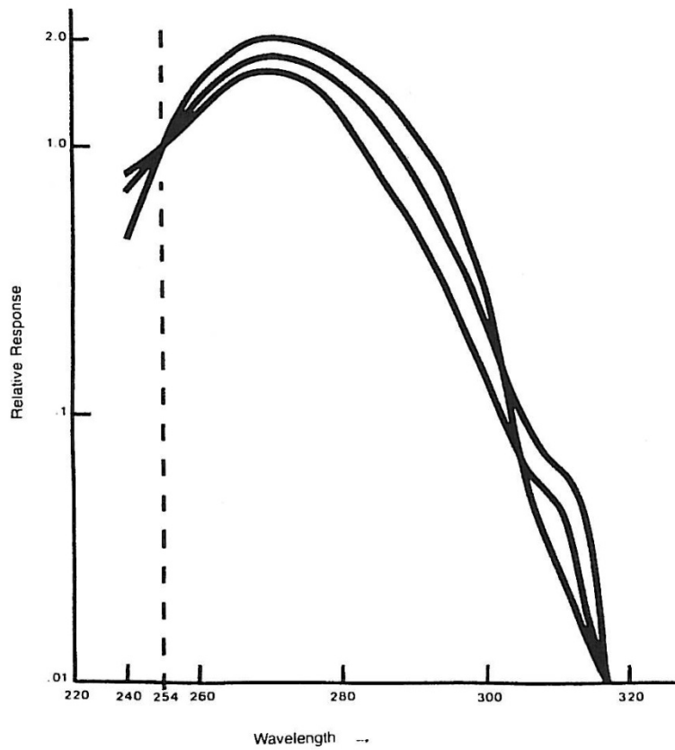
Figure 14: Response of Three Sensors Calibrated to Yield the Same Output at 254nm Wavelength
