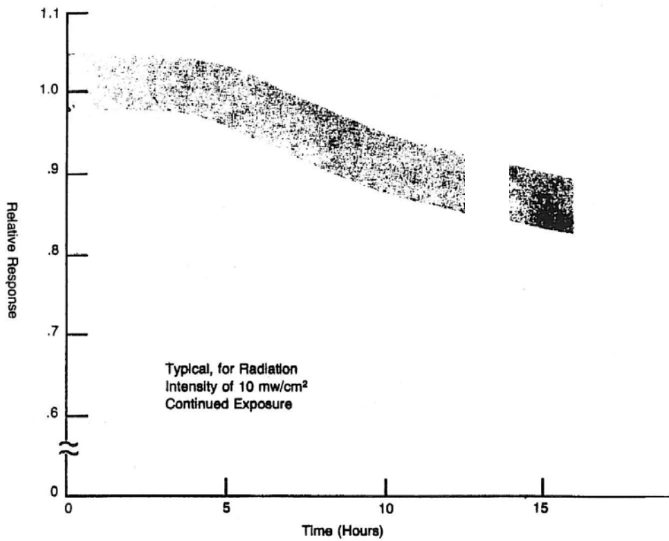
Figure 5: UVX-25 Sensor Solarization Curve
